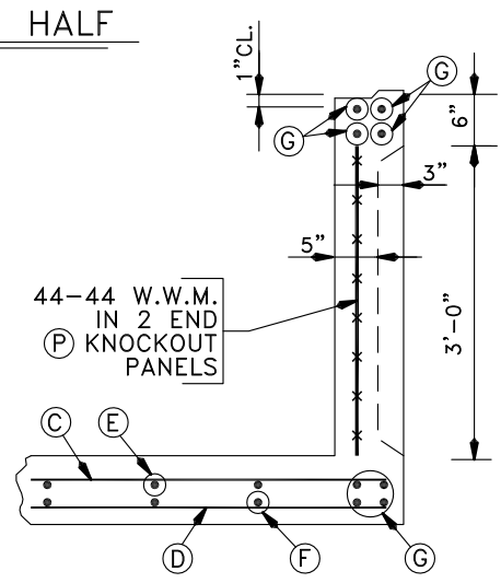
SECTION 2-2
