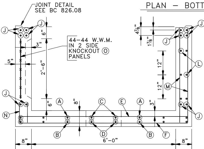
SECTION 1-1
