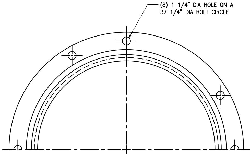
PARTIAL PLAN
